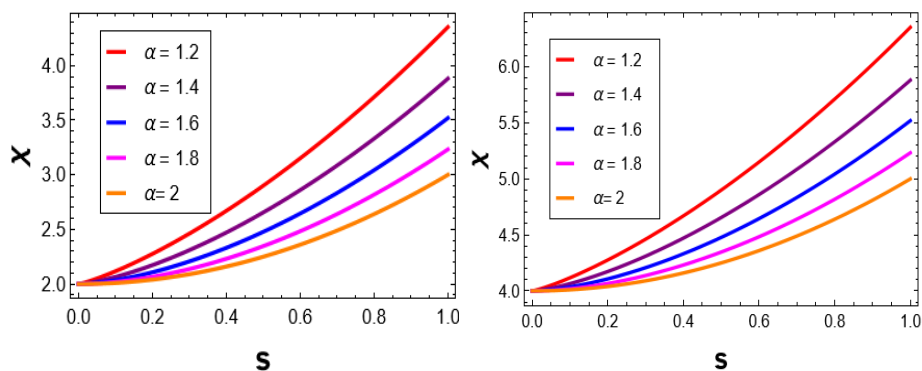
Figure 3. Exact solution to \chi(s, z) for \alpha = 1.2, 1.4, 1.6, 1.8, 2 with z = 2 and z = 4 , respectively.
