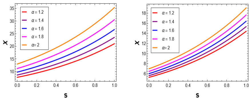
Figure 6. Exact solution to \chi(s, z) for \alpha = 1.2, 1.4, 1.6, 1.8, 2 with z = 2 and z = 3 , respectively.
