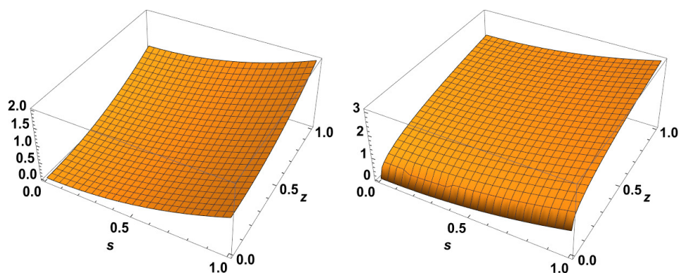
Figure 7. Exact solution to \chi(s, z) for \alpha = 2 and \alpha = 1.2 , respectively.
