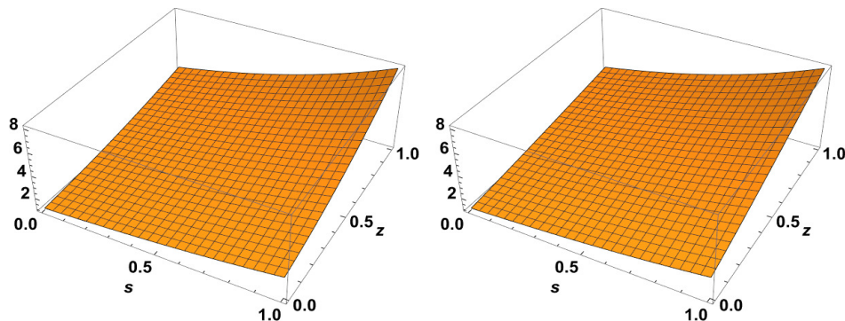
Figure 4. Exact solution to \chi(s, z) for \alpha = 2 and \alpha = 1.2 , respectively.
