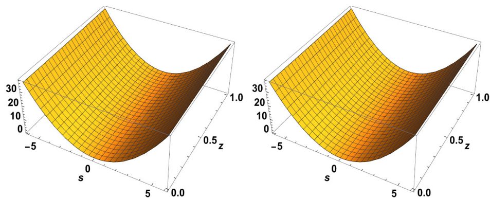
Figure 11. Exact solution to \chi(s, z) for \alpha = 1.4 and \alpha = 1.6 , k = 1 .
