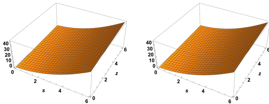
Figure 2. Exact solution to \chi(s, z) for \alpha = 1.4 and \alpha = 1.6 , respectively.
