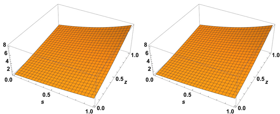
Figure 5. Exact solution to \chi(s, z) for \alpha = 1.4 and \alpha = 1.6 , respectively.
