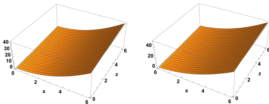
Figure 1. Exact solution to \chi(s, z) for \alpha = 2 and \alpha = 1.2 , respectively.
