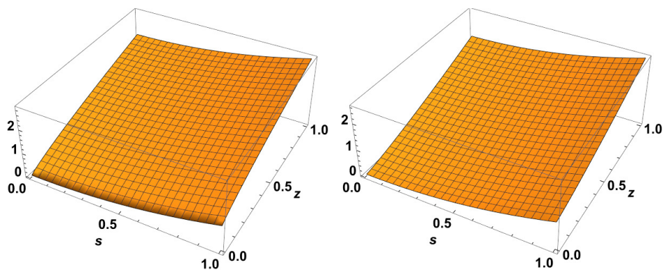
Figure 8. Exact solution to \chi(s, z) for \alpha = 1.4 and \alpha = 1.6 , respectively.
