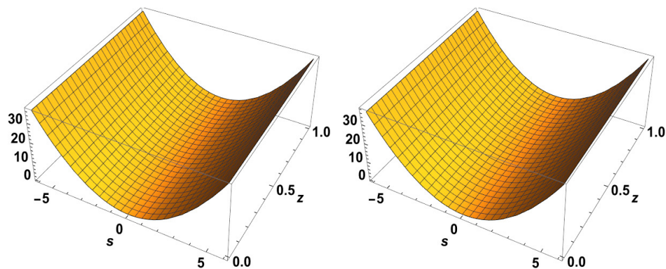
Figure 10. Exact solution to \chi(s, z) for \alpha = 2 and \alpha = 1.2 , k = 1 .
