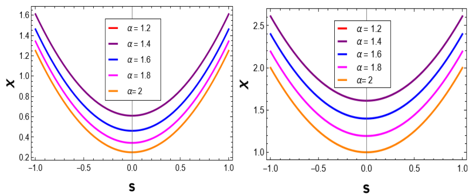
Figure 12. Exact solution to \chi(s, z) for \alpha = 1.2, 1.4, 1.6, 1.8, 2 with z = 0.5 and z = 1 , k = 1 .
