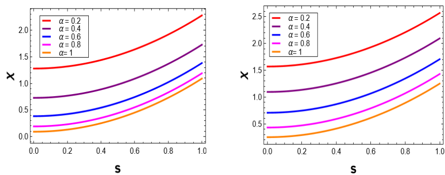
Figure 9. Exact solution to \chi(s, z) for \alpha = 0.2, 0.4, 0.6, 0.8, 1 with z = 0.3 and z = 0.5 , respectively.
