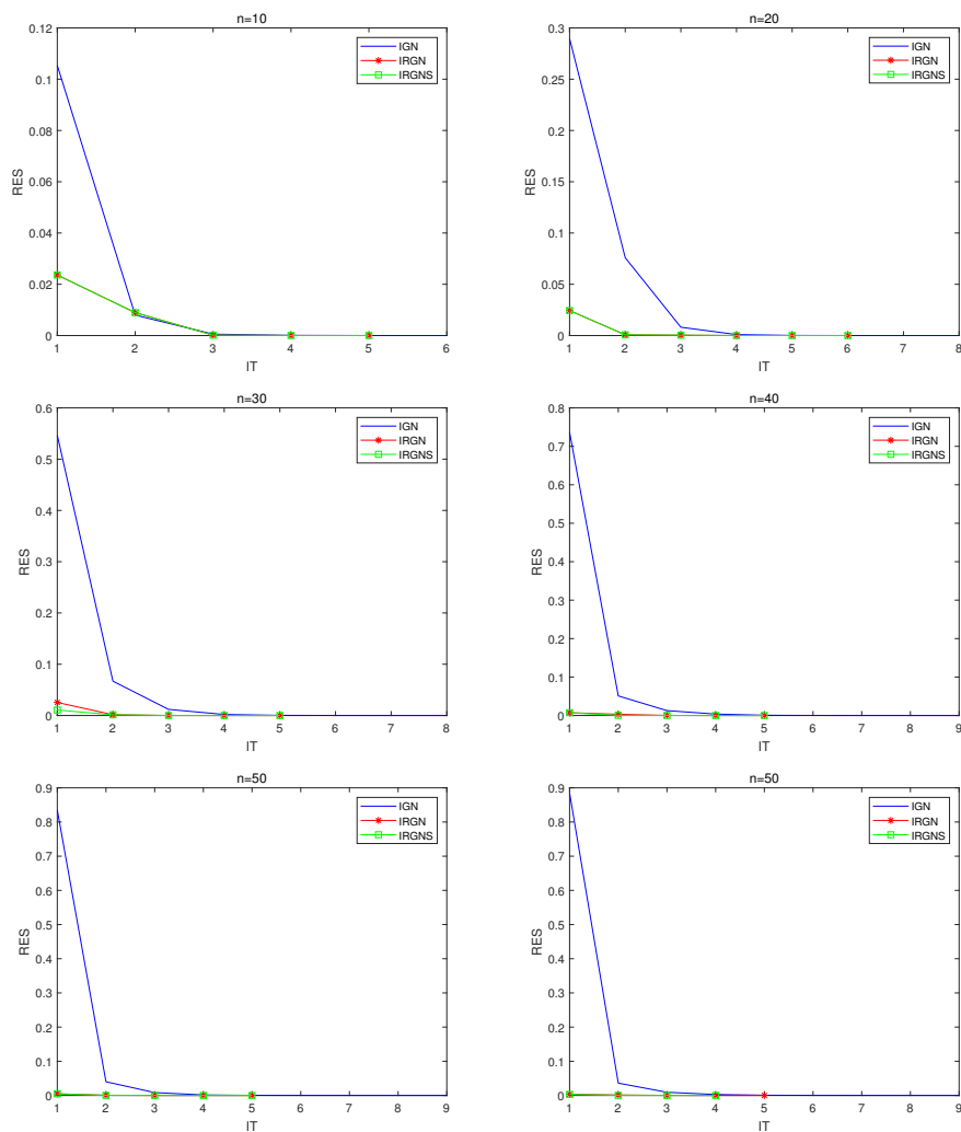
Figure 2. Convergence effect for Example 5.3
