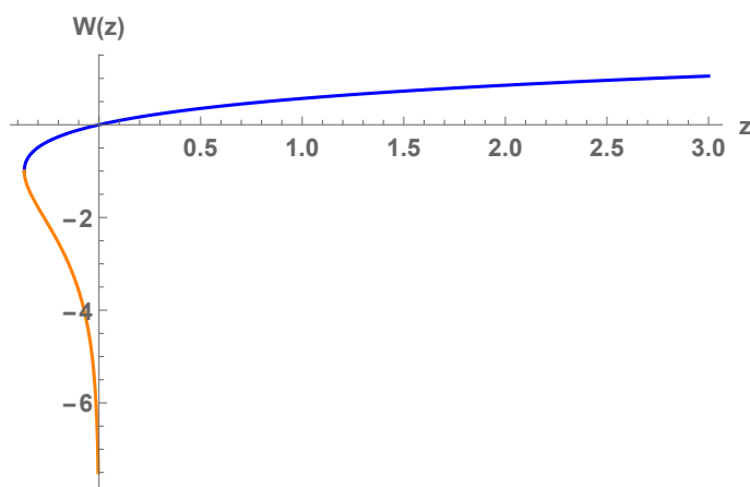
Figure 1. Branches W_{-1} (orange color) and W_0 (blue color) of the Lambert function (real solutions of we^w = z ). Both functions collide at z = -e^{-1} = -0.367879\dots
