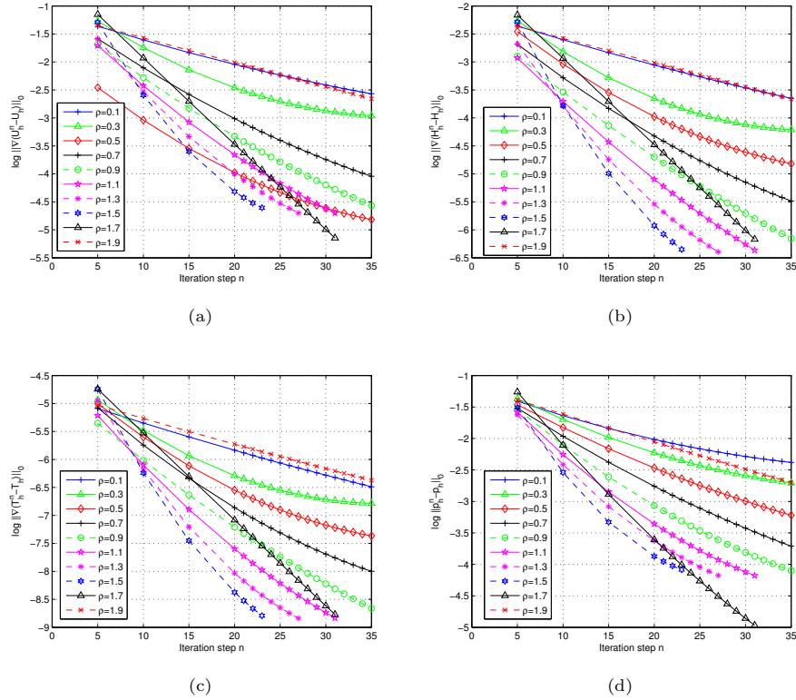
Figure 2. The log errors of the velocity (a), magnetic (b), temperature (c) and pressure (d) at the different iterative steps.
