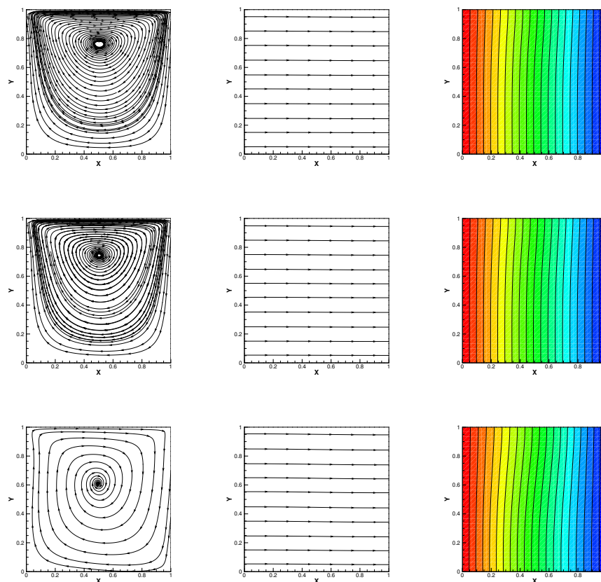
Figure 3. Numerical velocity streamlines, magnetic and isotherms with different thermal expansion coefficient \beta = 1 (the first line), \beta = 10 (the second line) and \beta = 100 (the third line).
