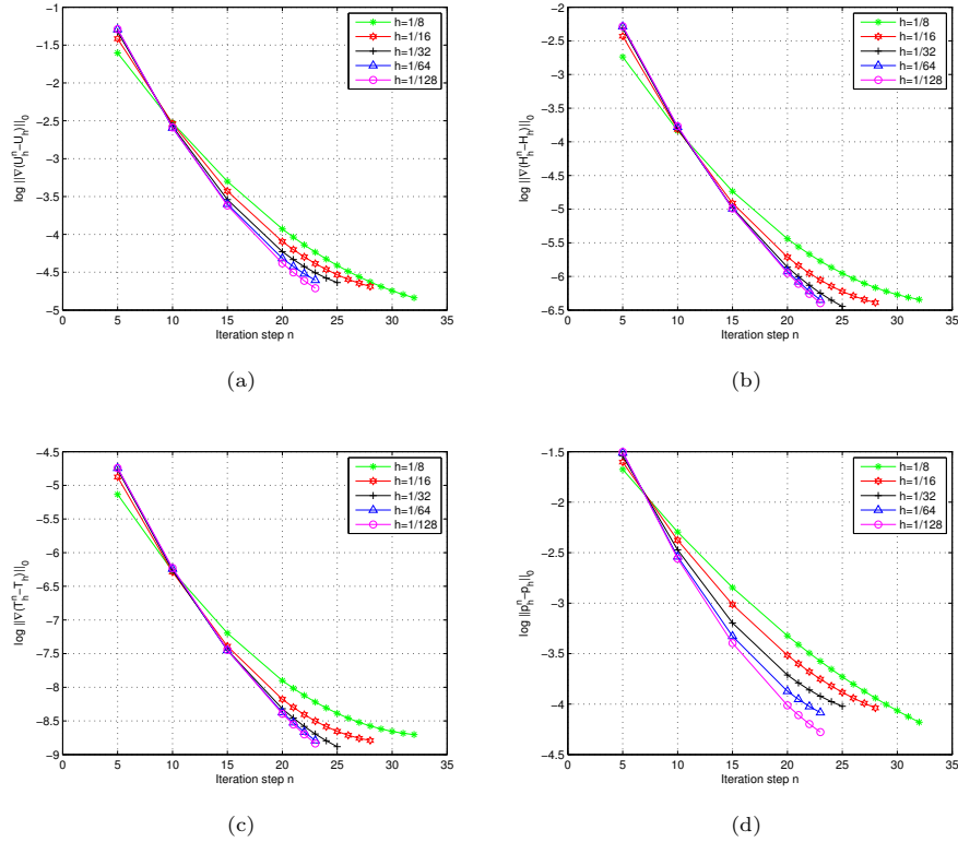
Figure 1. The log errors of the velocity (a), magnetic (b), temperature (c) and pressure (d) at the different iterative steps.
